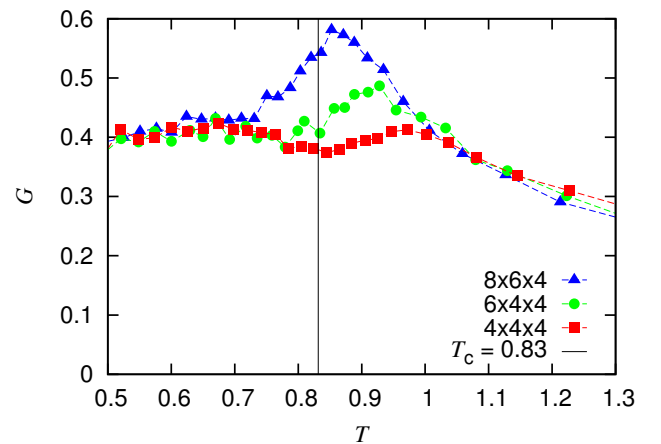
FIG. 10: Temperature dependences of the G -index for the Heisenberg model on lattices of three different sizes indicated in the figure.
