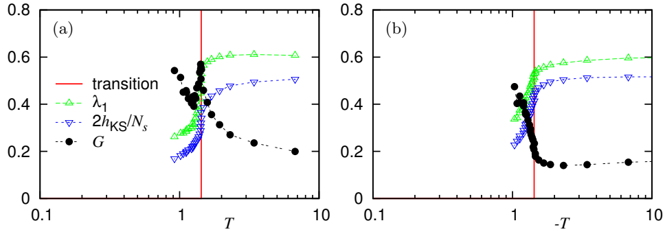
FIG. 11: Lyapunov exponents and G -index as functions of temperature for several different sets of coupling constants (indicated above the plots). The position of the phase transition is indicated with a red vertical line. (J_x, J_y, J_z) = (4, 2, 1)/\sqrt{21} \approx (0.873, 0.436, 0.218) .
