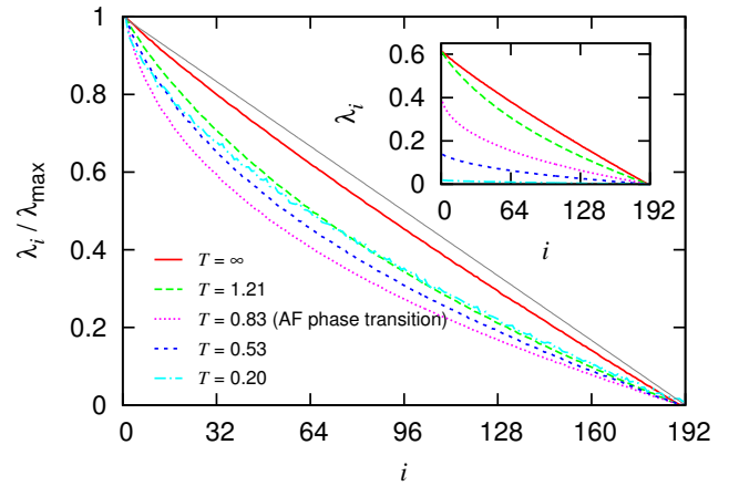
FIG. 3: Examples of Lyapunov spectra for the lattice used for Fig. 2. The thin gray straight line extending along the diagonal of the main plot is drawn to illustrate the geometrical interpretation of the G -index given in the text.
