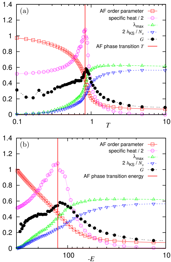
FIG. 2: Specific heat, AF order parameter, the largest Lyapunov exponent, Kolmogorov-Sinai entropy and the G -index as functions of (a) temperature and (b) energy for the 8 \times 6 \times 4 lattice with Heisenberg interaction J_x = J_y = J_z = 1/\sqrt{3} . The positions of the AF phase transition are indicated by the vertical lines.
