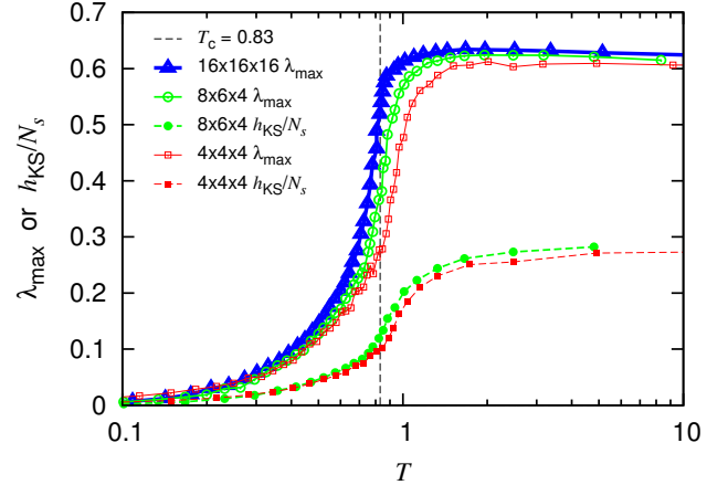
FIG. 9: The same quantities as in Fig. 8 but plotted as functions of temperature, for E < 0 .
