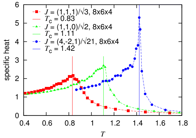
FIG. 1: Temperature dependence of the specific heat for three different lattices in the vicinity of their respective phase transitions. We identify the phase transition as the point of maximum specific heat.
