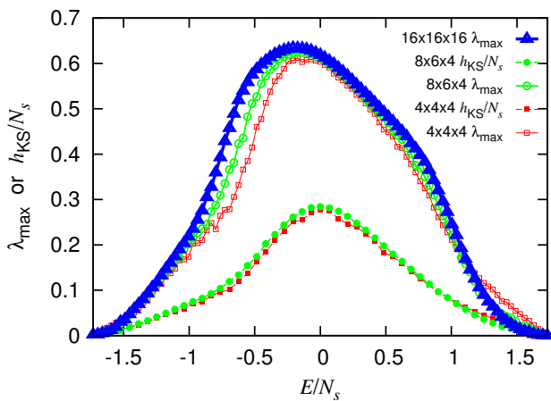
FIG. 8: The largest Lyapunov exponent and Kolmogorov-Sinai entropy per spin of the Heisenberg model for several different lattice sizes as functions of the energy per spin. The Kolmogorov-Sinai entropy for the 16 \times 16 \times 16 system is not shown, as it is impossible to obtain sufficiently accurately with currently available computing power. Even for the largest system, the Lyapunov exponents and Kolmogorov-Sinai entropy depend smoothly on the energy.
