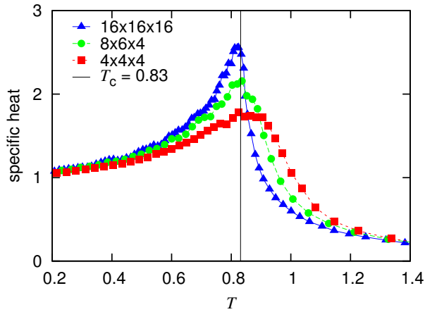
FIG. 7: Specific heat of the Heisenberg model for lattices of different sizes indicated in the figure.
