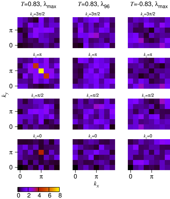
FIG. 5: Spectral functions F(k_x, k_y, k_z) of three Lyapunov vectors for the lattice with Heisenberg interaction used for Figs. 4 (a) and (b). The left and the middle columns of frames represent F(k_x, k_y, k_z) for the Lyapunov vectors corresponding to \lambda_{\max} and \lambda_{96} , respectively, at the AF transition temperature. The right column corresponds to the Lyapunov vector for \lambda_{\max} at the FM transition temperature. Each column shows a complete set of values of F(k_x, k_y, k_z) encoded as color pixels: one pixel for each of 8 \times 6 \times 4 possible combinations of wave numbers (k_x, k_y, k_z) . Each frame contains 8 \times 6 pixels for a fixed value of k_z indicated above the frame.
