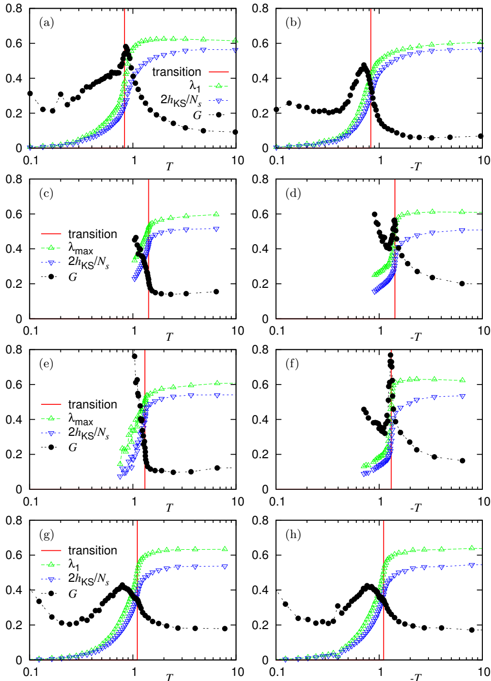
FIG. 4: Indicators of the phase transition and dynamic quantities as a function of temperature, for Heisenberg coupling and two types of anisotropic coupling. For (a) and (b) (J_x, J_y, J_z) = (1, 1, 1)/\sqrt{3} \approx (0.577, 0.577, 0.577) , for (c) and (d) (J_x, J_y, J_z) = (4, -2, 1)/\sqrt{21} \approx (0.873, -0.436, 0.218) , for (e) and (f) (J_x, J_y, J_z) = (2, -1, 1)/\sqrt{6} \approx (0.816, -0.408, 0.408) , and for (g) and (h) (J_x, J_y, J_z) = (1, 1, 0)/\sqrt{2} \approx (0.707, 0.707, 0.0) . The coupling constants are indicated above the plots. Both the AF and the FM sides are shown. Below some transitions, formation of magnetic domains prevents the averages and Lyapunov exponents from converging sufficiently within the simulation time.
