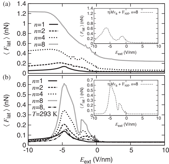
FIG. 5. The friction force as a function of the external field for extended commensurate tips of different sizes and with lattice spacing commensurate b = a (a) and incommensurate b = \lambda a (b) with the dipole array. The insets show the contributions from dipole rotation for the case of n = 8 . For larger commensurate tips the high barrier dominates the friction force, while for incommensurate tips the dipole rotation dominates the friction force.
