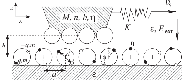
FIG. 1. Sketch of the model. A tip is dragged over a surface covered by a monolayer of polar molecules, in the presence of an external electric field E_{\text{ext}} .
