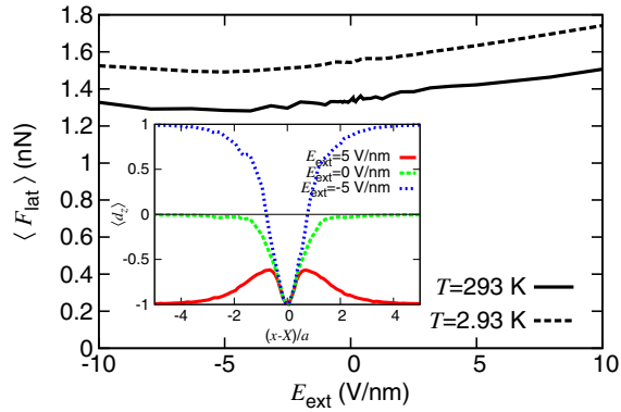
FIG. 3 (color online). Friction characteristics for a system with purely electrostatic interactions: the friction force as a function of the field strength for two different temperatures, and (inset) the average dipole orientation as a function of the distance of the dipoles from the tip for three different fields strengths at T = 2.93\text{ K} .
