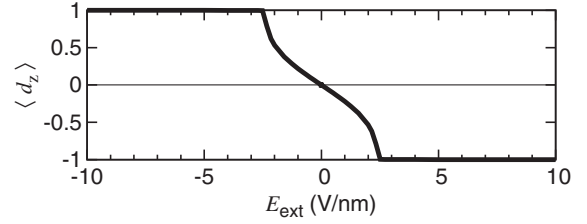
FIG. 2. Dependence of the average z component of the unit vector along the dipole direction, \langle d_z \rangle = \cos \phi , on the electric field for a system of 512 dipoles equilibrated at T = 2.93 K without the tip.
