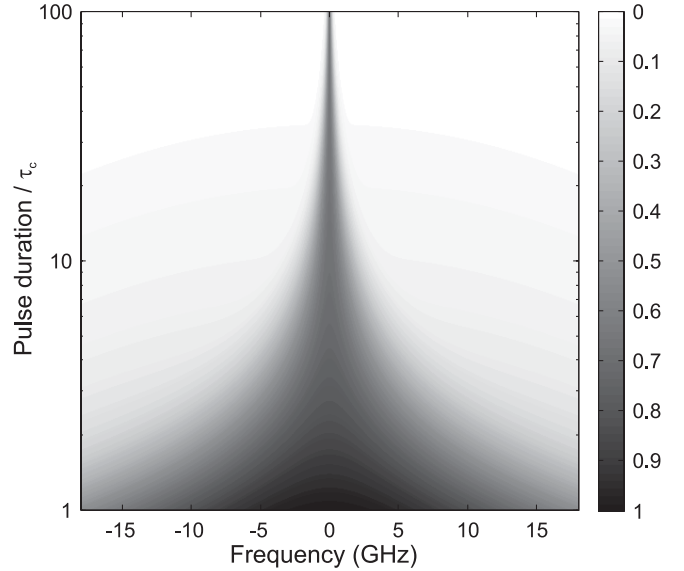
FIG. 3. Normalized amplitude of the forcing spectrum for zero delay as a function of pump laser pulse duration. The amplitude is plotted in a linear gray scale; pump pulse duration in units of the coherence time, \tau_c = 12 ps, is logarithmic.
